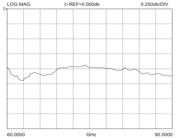
S21 FORWARD TRANSMISSION
