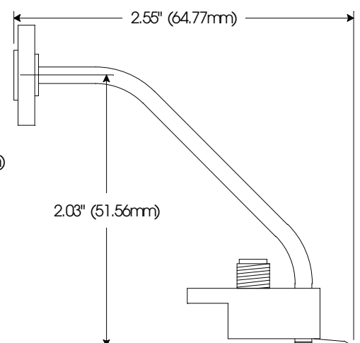
Model 75-BT-M Waveguide Dimensions
