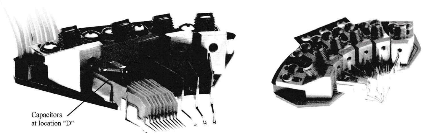
Two examples of the Picoprobe® Multi-Contact Wedge
