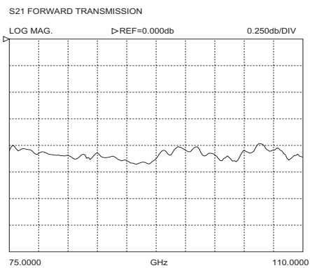
Typical insertion loss of a Model 120-GSG-150-BT
